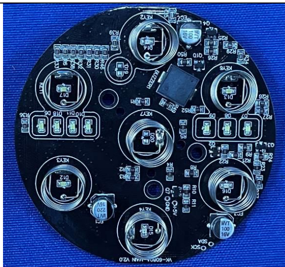
Control PCB 3#
